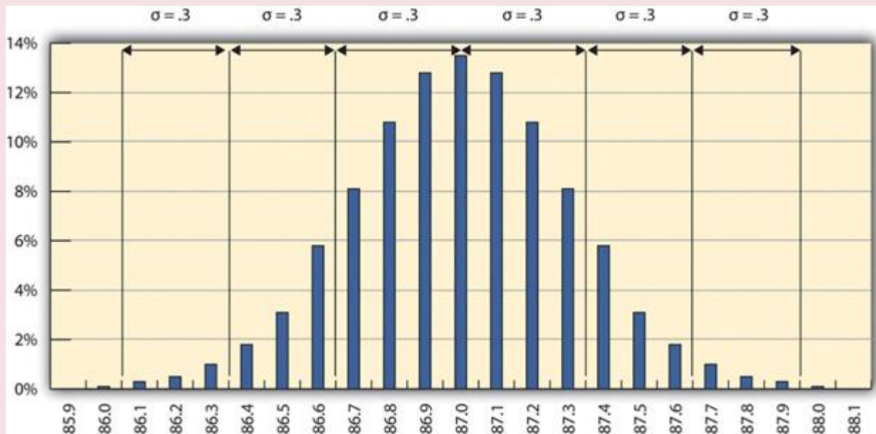
Figure 14.3 The 68-95-99.7 Rule
