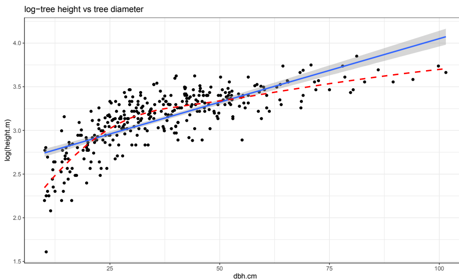
Figure 7.14: Scatterplot of \log(\text{tree height}) versus tree diameter.
