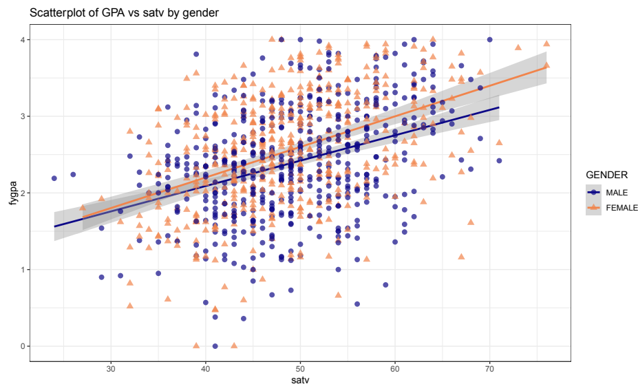
Figure 8.22: Plot of fygpa vs satv by gender of students.
