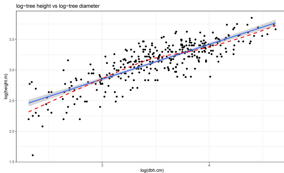
Figure 7.16: Scatterplot of log(tree height) versus log(tree diameter).
