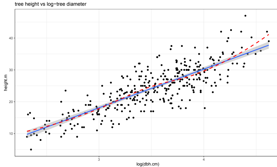
Figure 7.15: Scatterplot of tree height versus log(tree diameter).
