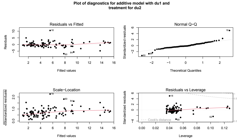
Figure 8.29: Diagnostic plots for the additive decibel tolerance model.
