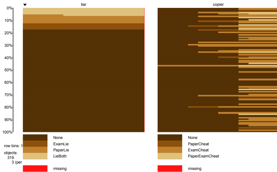
Figure 5.19: Tableplot of new variables liar and copier that allow exploration of relationships between different types of lying and cheating behaviors.
