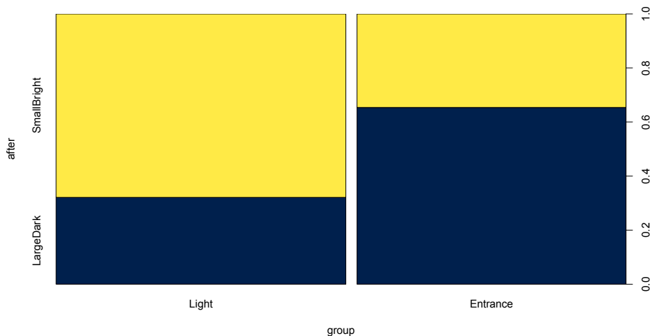
Figure 9.9: Stacked bar chart for Ant Colony results.
