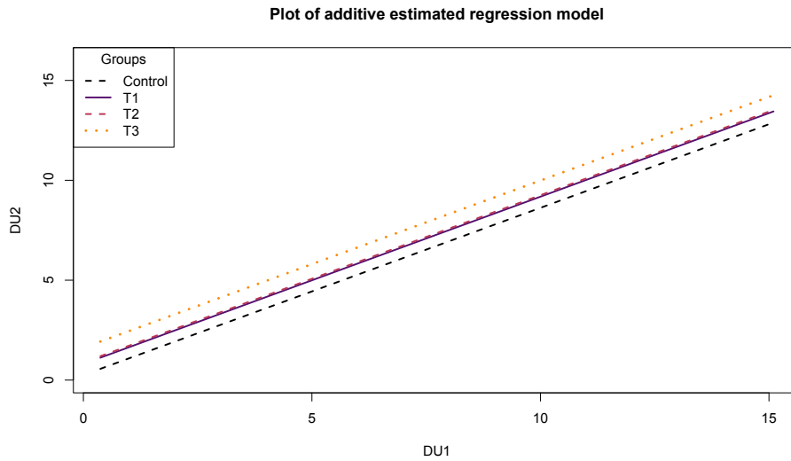
Figure 8.27: Plot of estimated noise tolerance additive model.
