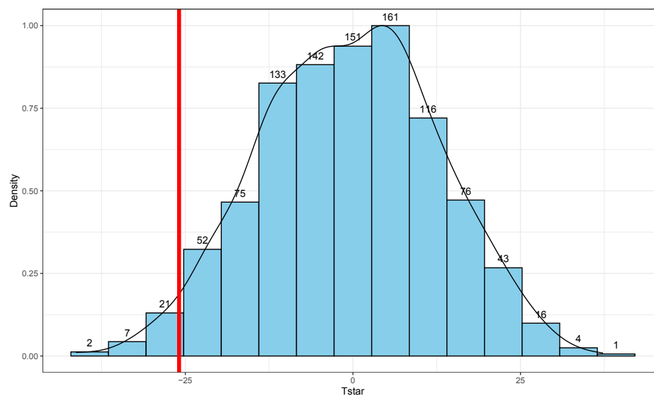
Figure 2.9: Histogram and density curve of values of test statistic for 1,000 permutations with bold vertical line for the value of observed test statistic.
