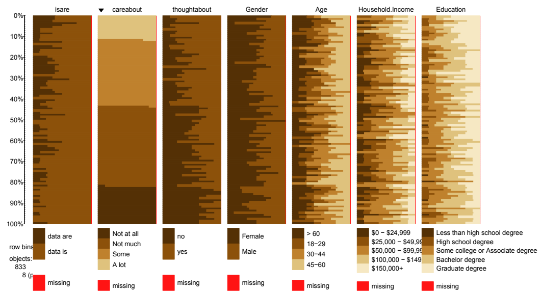
Figure 5.27: Tableplot of data from “data-is-vs-data-are” survey, sorted by “CareAbout” responses.
