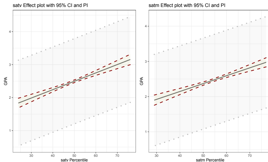
Figure 8.21: Term-plots for the fgpa \sim satv + satm model with 95% confidence intervals (dark, dashed lines) and 95% PIs (light grey, dotted lines).
