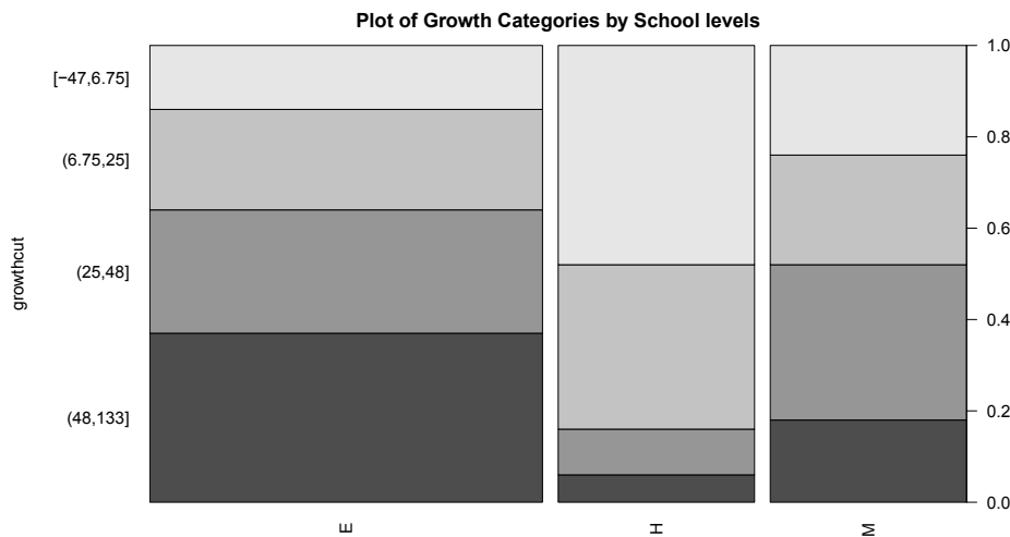
Figure 5.25: Stacked bar chart of the growth stype category responses by level of school.
