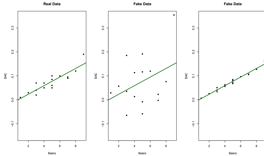
Figure 6.19: Three scatterplots with the same estimated regression line.
