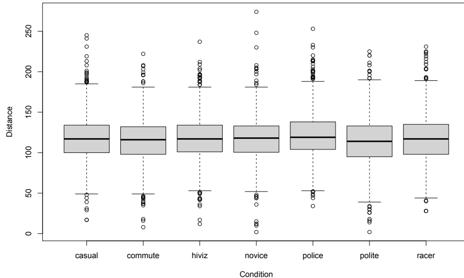
Figure 2.3: Side-by-side boxplot of distances based on outfits.
