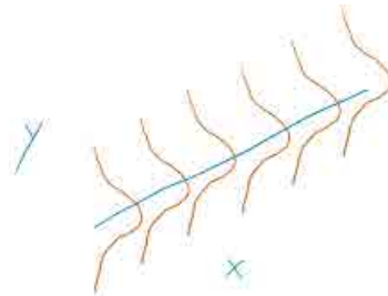
Figure 7.1: Sketch of assumed normal distributions for the responses centered at the regression line.
