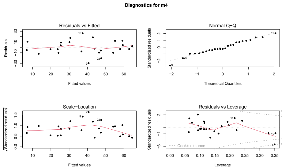
Figure 8.6: Diagnostic plots for model m4: \text{Snow.Depth} \sim \text{Elevation} + \text{Min.Temp} + \text{Max.Temp} .
