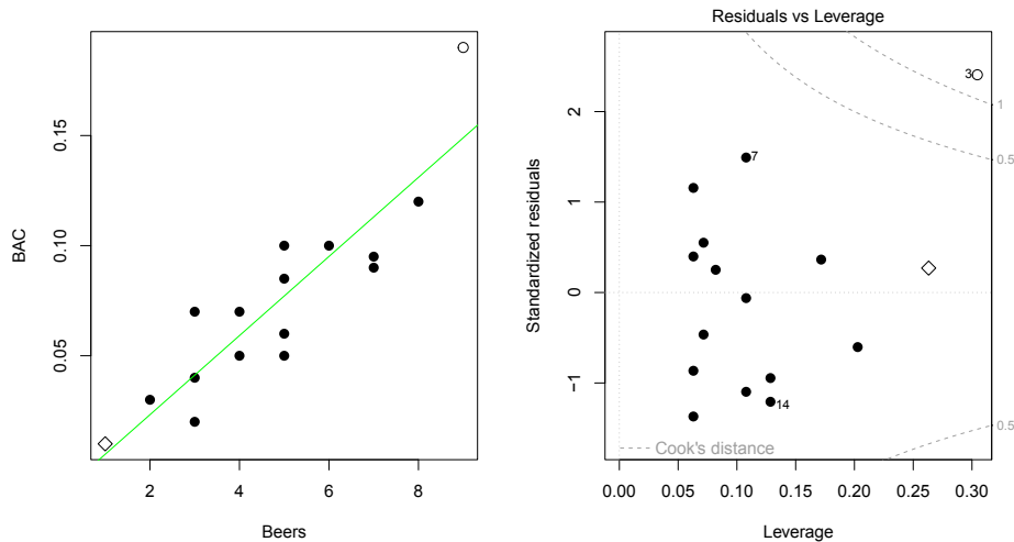
Figure 6.20: Scatterplot and Residuals vs Leverage plot for the real BAC data. Two high leverage points are flagged, with only one that has a Cook's D value over 1 (“○”) and is indicated as influential.
