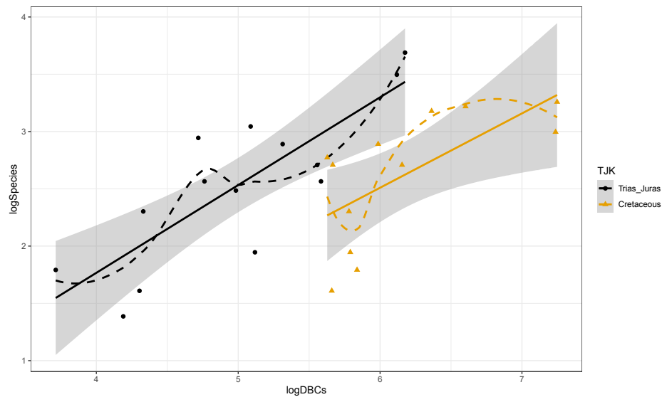
Figure 9.10: Scatterplot of \log -biodiversity vs \log -DBC by TJK .
