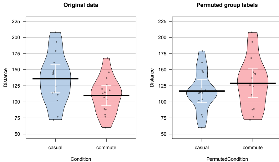
Figure 2.7: Violin-plots of Distance responses versus actual treatment groups and permuted groups. Note how the responses are the same but that they are shuffled between the two groups differently in the permuted data set. With the smaller sample size, the 95% confidence intervals for each of the means are more clearly visible than with the original large data set.
