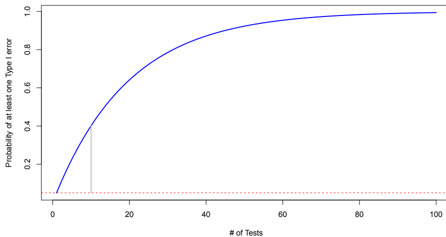
Figure 2.20: Plot of family-wise error rate (bold solid line) as the number of tests performed increases. Dashed line indicates 0.05 and grey solid line highlights the probability of at least one error on m = 10 tests.
