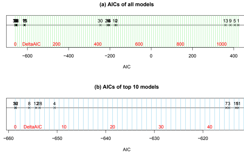
Figure 8.45: Display of AIC results on a number line with models indicated by their number in the dredge output. In more complex models, the dredge model numbers are just labels and not a meaningful numeration of the models being considered (there are 20 models considered here but labels go up to 32). Panel (a) presents results for all the models and panel (b) focuses just on the top 10 models so some differences in those models can be explored. Note that the spacing of the vertical grid lines in panel (a) are 10 AIC units and in (b) they are 1 AIC unit apart.
