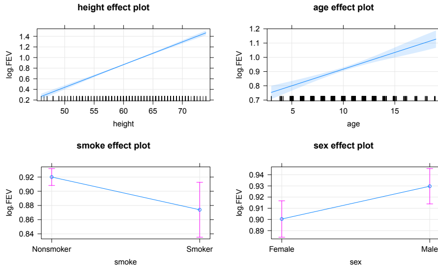
Figure 8.46: Term-plots for the top AIC model for log(FEV) that includes height, age, smoking status, and sex in the model.
