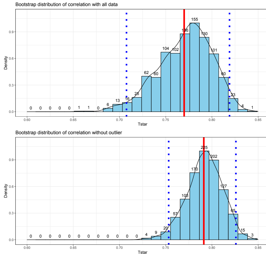
Figure 6.12: Bootstrap distributions of the correlation coefficient for the full data set (top) and without potential outlier included (bottom) with observed correlation (bold line) and bounds for the 95% confidence interval (dashed lines). Notice the change in spread of the bootstrap distributions as well as the different centers.
