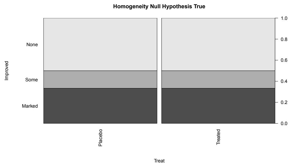
Figure 5.4: Stacked bar chart of one way that the Arthritis proportions could have been if the null hypothesis had been true.
