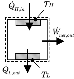
Figure 8-4 Power cycle operating between T_H and T_L .
