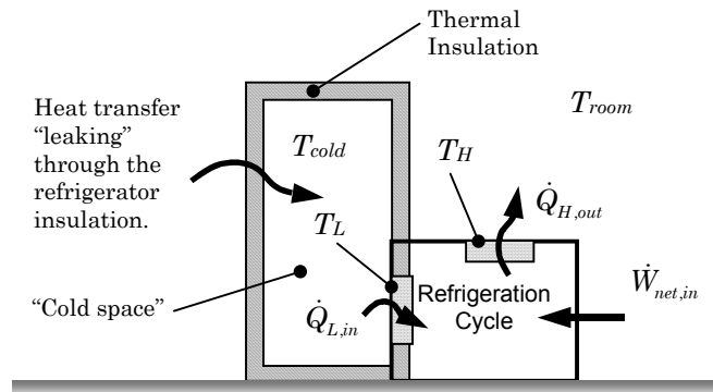
Figure 8-6 How a refrigeration cycle is used to keep the inside of a refrigerator or freezer cold.
