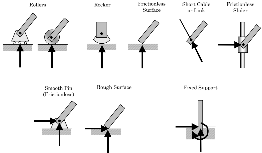
Figure 6-11 Surface Force Reactions
