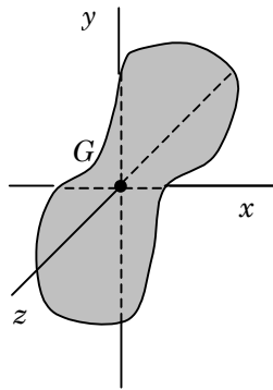
Figure 6-9 Moment of inertia of a mass
