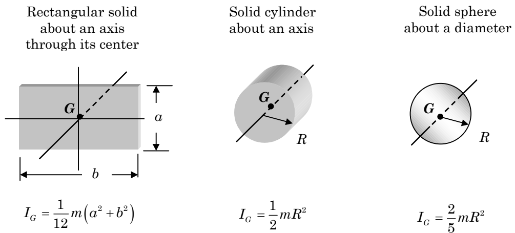
Figure 6-10 Centroidal mass moment of inertia for some common shapes
