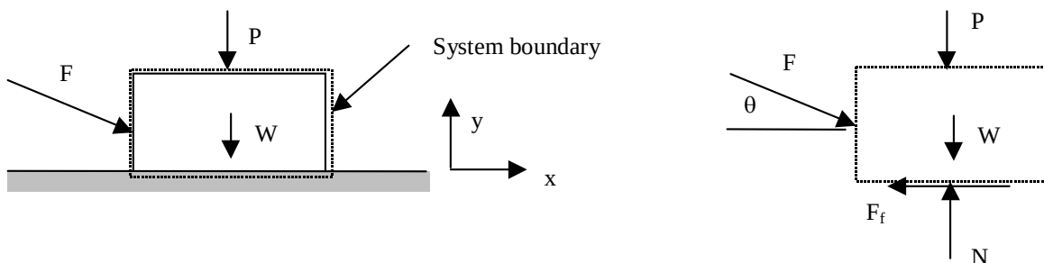
Figure 5-15 Block moving on a horizontal surface with friction
