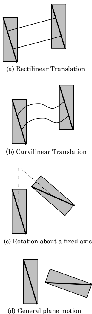
Figure 5-5 Plane motion of a rigid body
