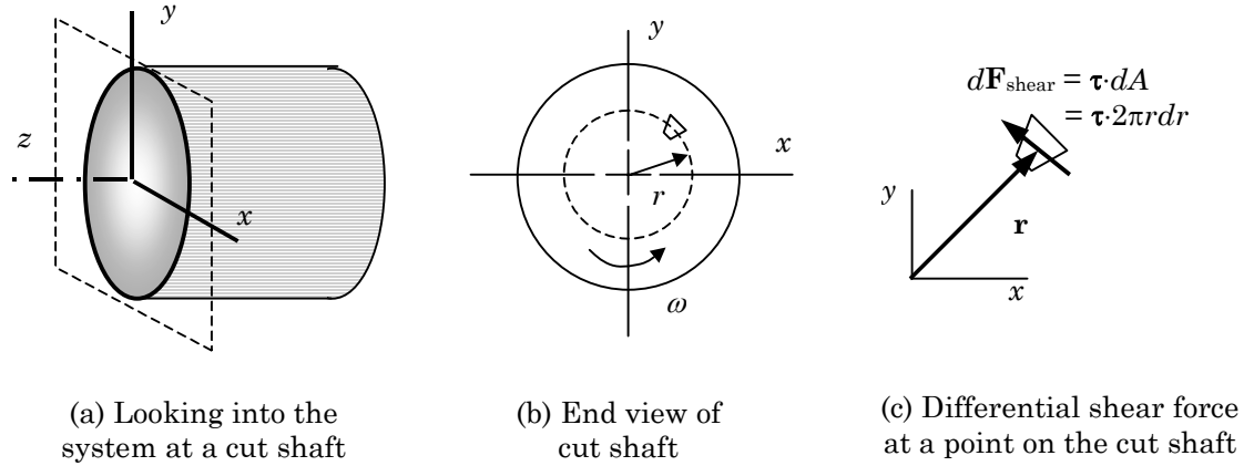
Figure 7-9 View into a system containing a rotating shaft
