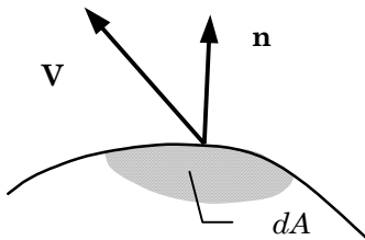
Figure 5-14 Mass transport of linear momentum at a boundary
