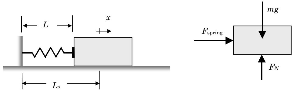
Figure 7-5 Forces acting on a block by an expanding spring.
