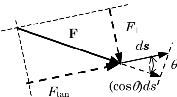
Figure 7-2 Evaluating differential mechanical work, \delta W_{\text{mech}}
