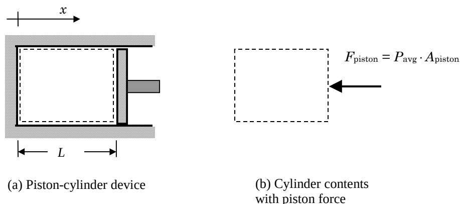
Figure 7-8 Compression-Expansion Work for a Piston-Cylinder Device
