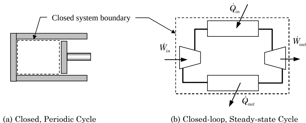
Figure 7-23 Classification of thermodynamic cycles by physical structure
