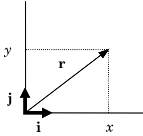
Figure 5-3 Rectangular Coordinates
