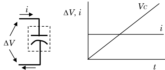
Figure 7-20 Voltage-current relationship for an ideal capacitor.
