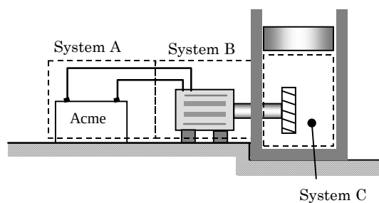
Figure 7-7 Examples of work transfer of energy
