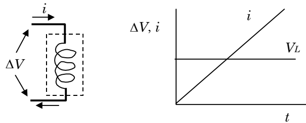
Figure 7-21 Voltage–current relationship for an ideal inductor.
