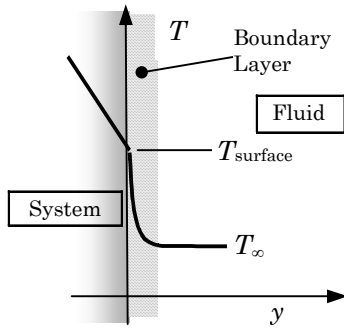
Figure 8-3 Entropy production at a system boundary with convection heat transfer
