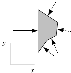
Figure 5-12 Pressure forces using projected areas.
