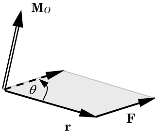
Figure 6-3 Sense of direction of \mathbf{M}_O using the right-hand rule
