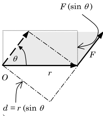
Figure 6-4 Interpreting the magnitude of \mathbf{M}_O as an area.
