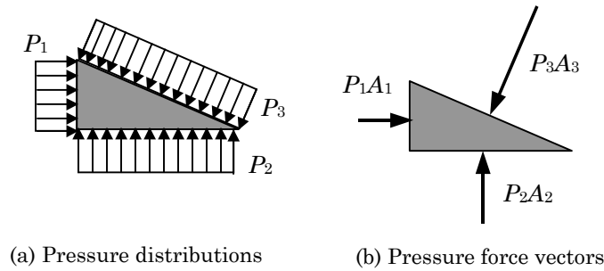
Figure 5-11 Forces due to uniform pressure
