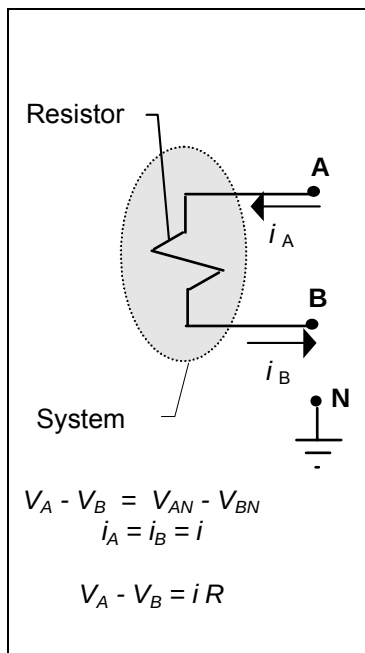
Figure 4-1 Resistor
