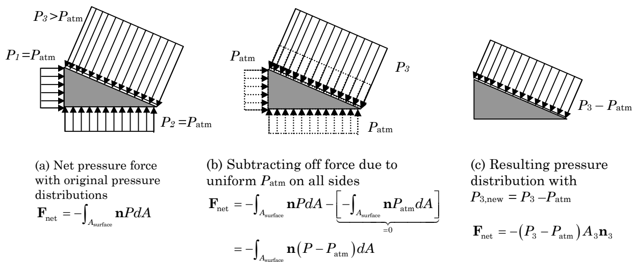
Figure 5-13 Calculating net pressure force when most of the system sees atmospheric pressure.
