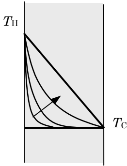
Figure 7-15 Temperature profile for transient conduction in a plane wall.
