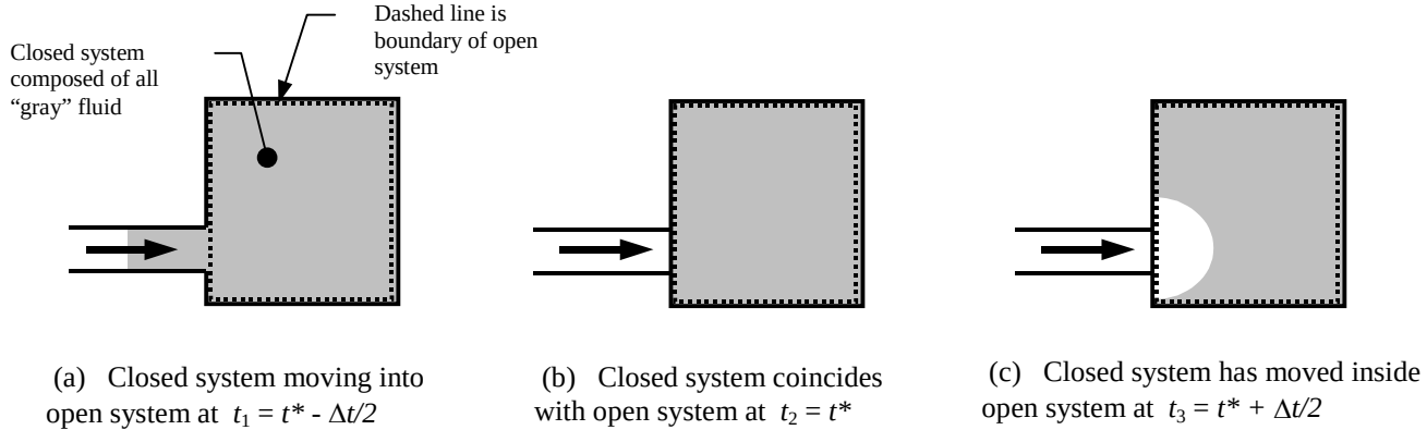
Figure 7-13 - Flow of a closed system into an open system
