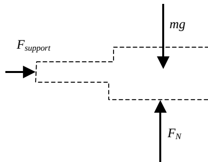
Figure 7-6 Analyzing a system with the spring inside the system.
