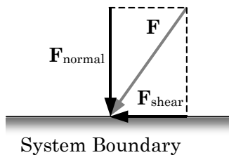
Figure 5-9 Normal and Shear Forces
