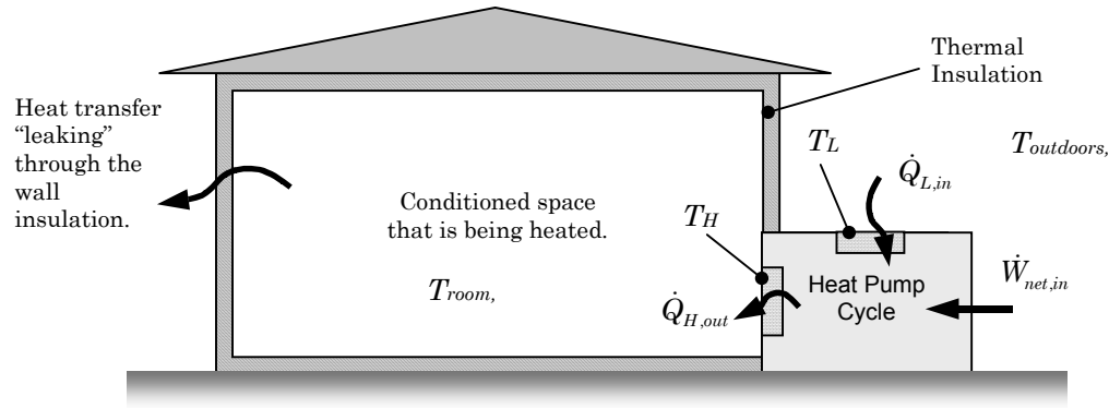
Figure 8-7 How a heat pump cycle is used to heat a house.
