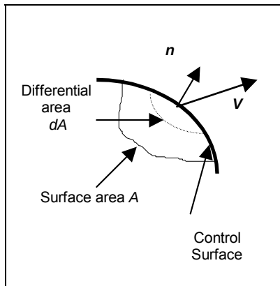
Figure 3-2 Geometry for flow across a system boundary.
