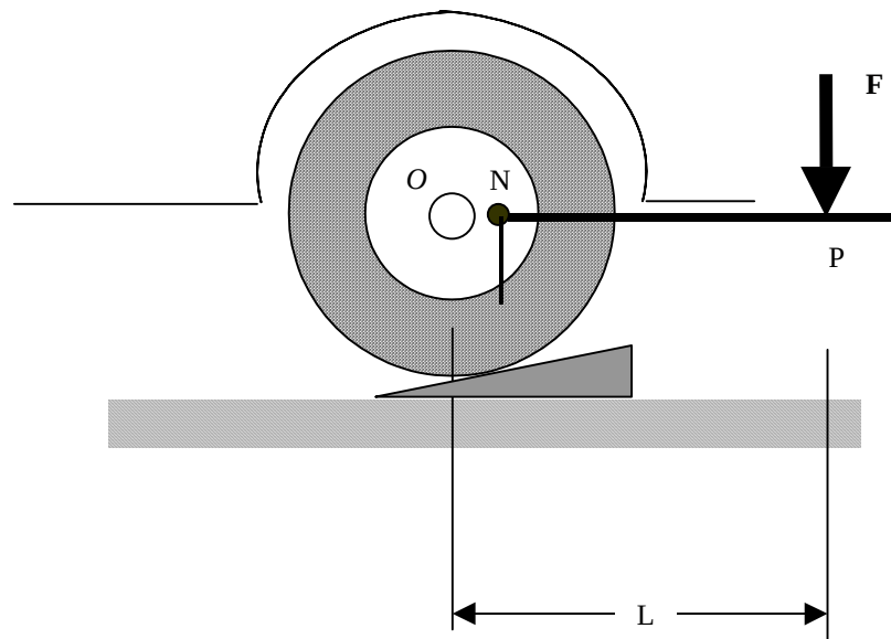
Figure 6-1 Changing a tire
