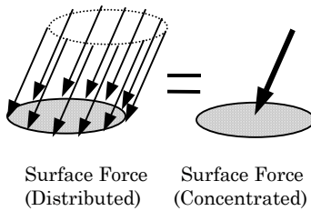
Figure 5-8 Surface forces
